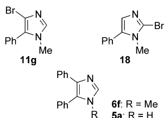
Figure 1. Chemical structures of 11g , 18 , 6f , and 5a .
