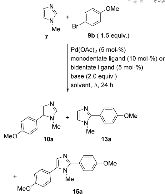
Scheme 2.
